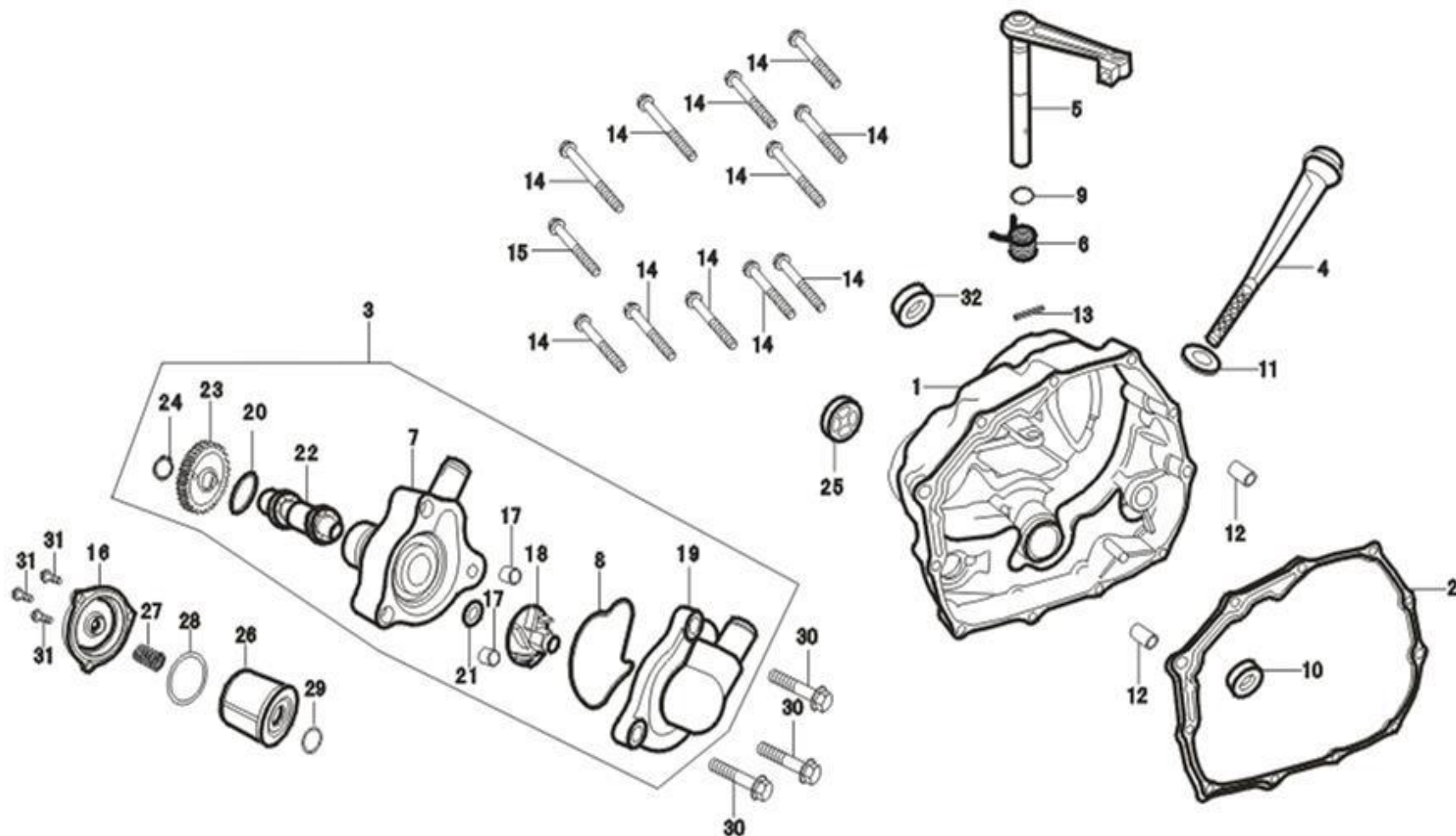
3504... (RIGHT CRANKCASE COVER)
